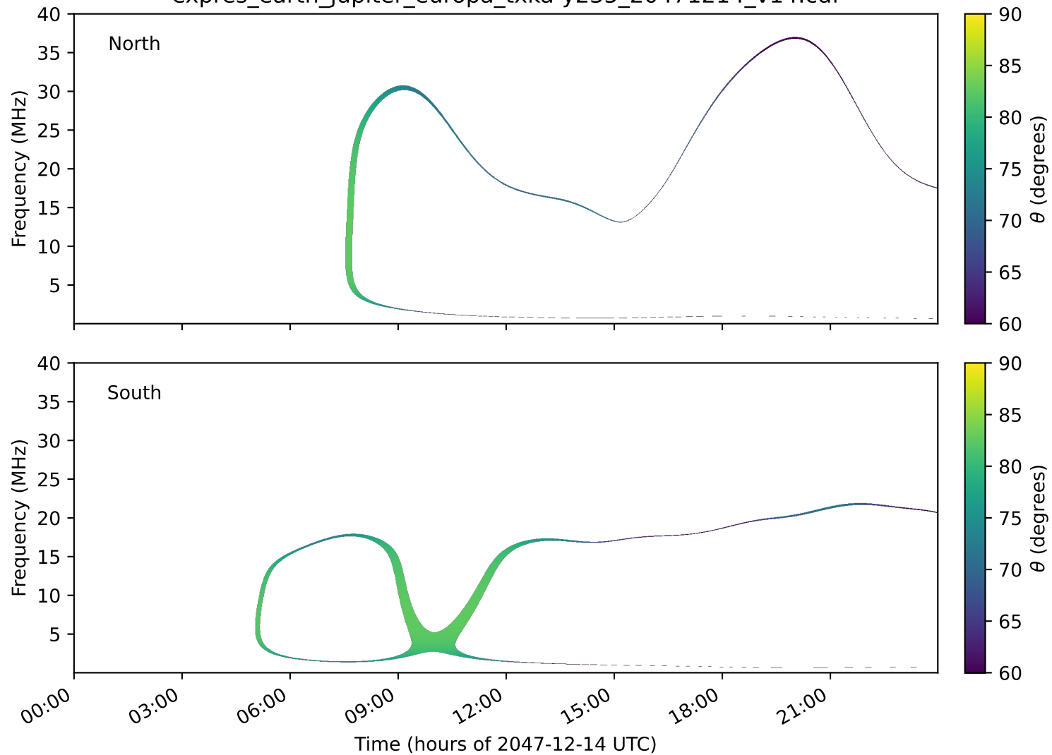
expres_earth_jupiter_europa_txka-y235_20471214_v14.cdf
