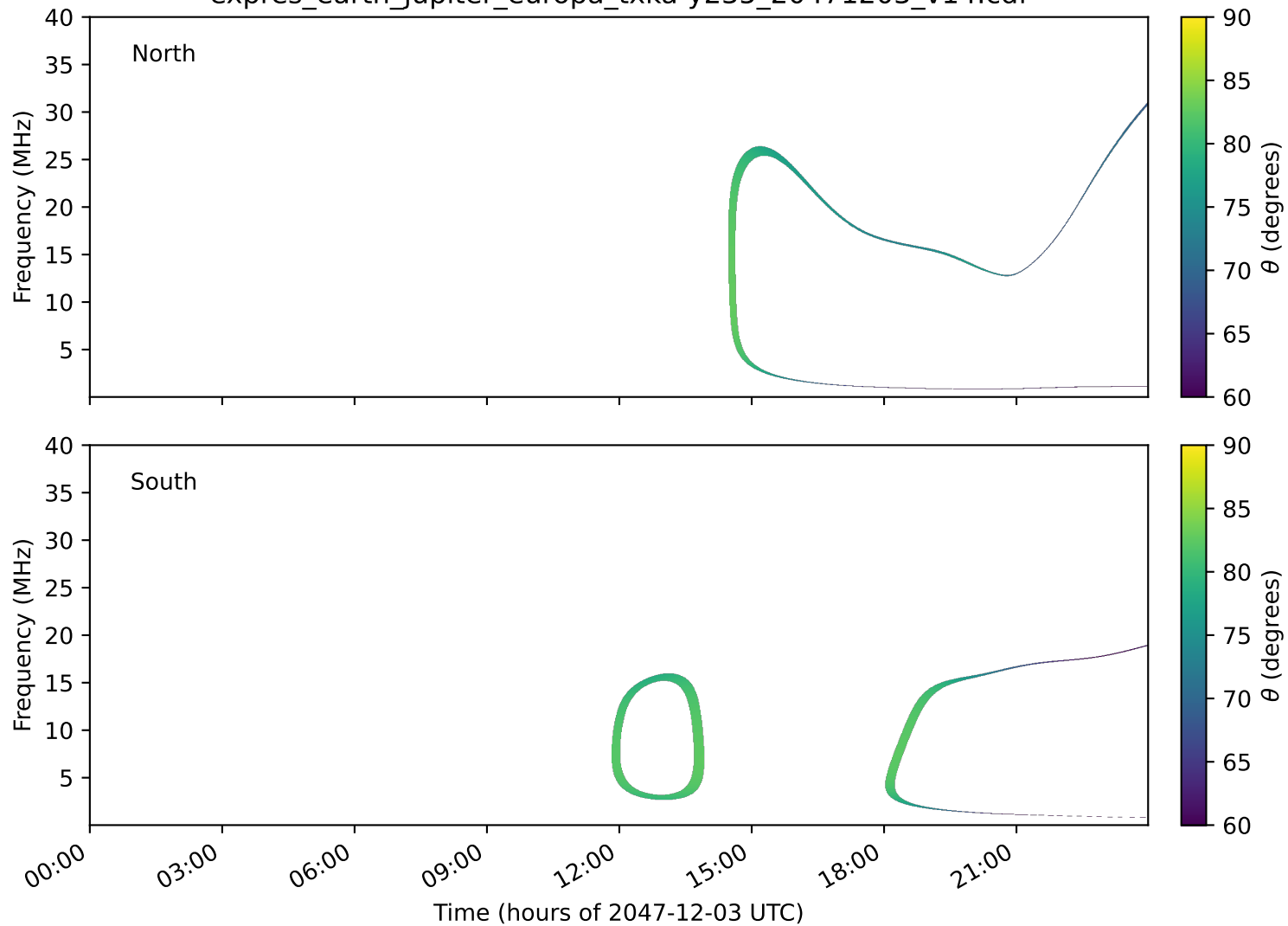
expres_earth_jupiter_europa_txka-y235_20471203_v14.cdf
