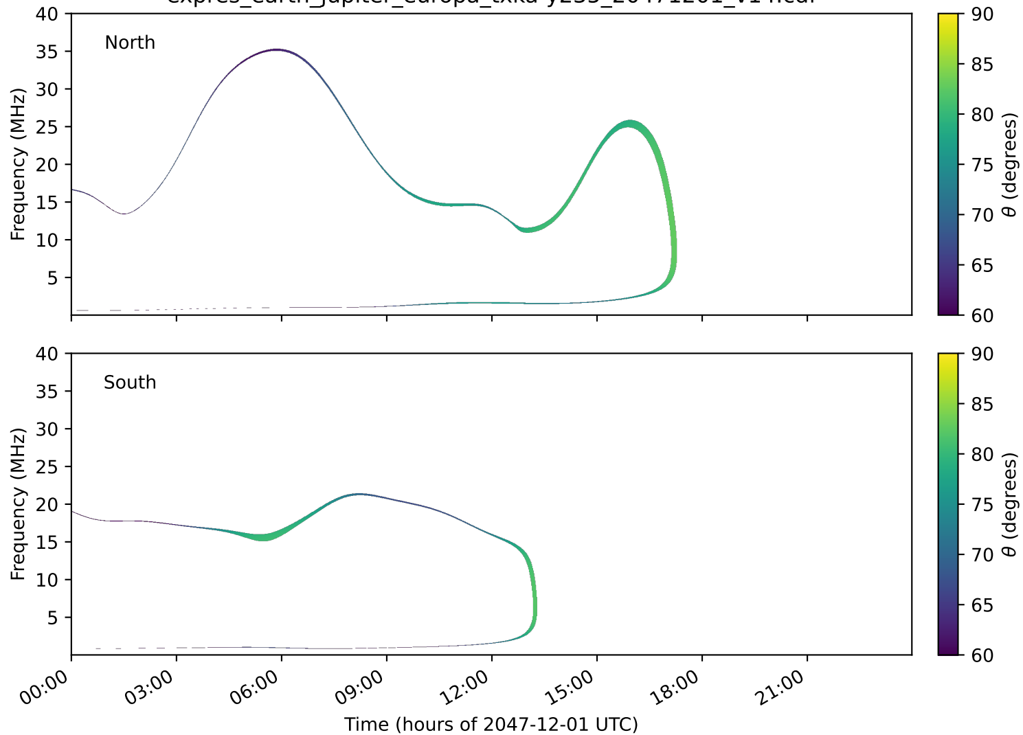
expres_earth_jupiter_europa_txka-y235_20471201_v14.cdf
