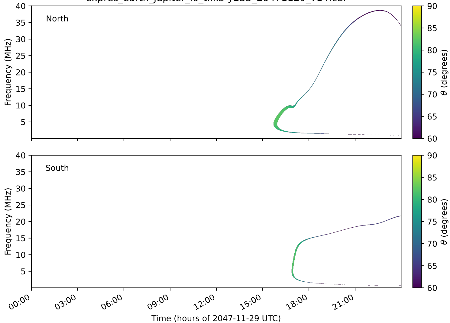
expres_earth_jupiter_io_txka-y235_20471129_v14.cdf
