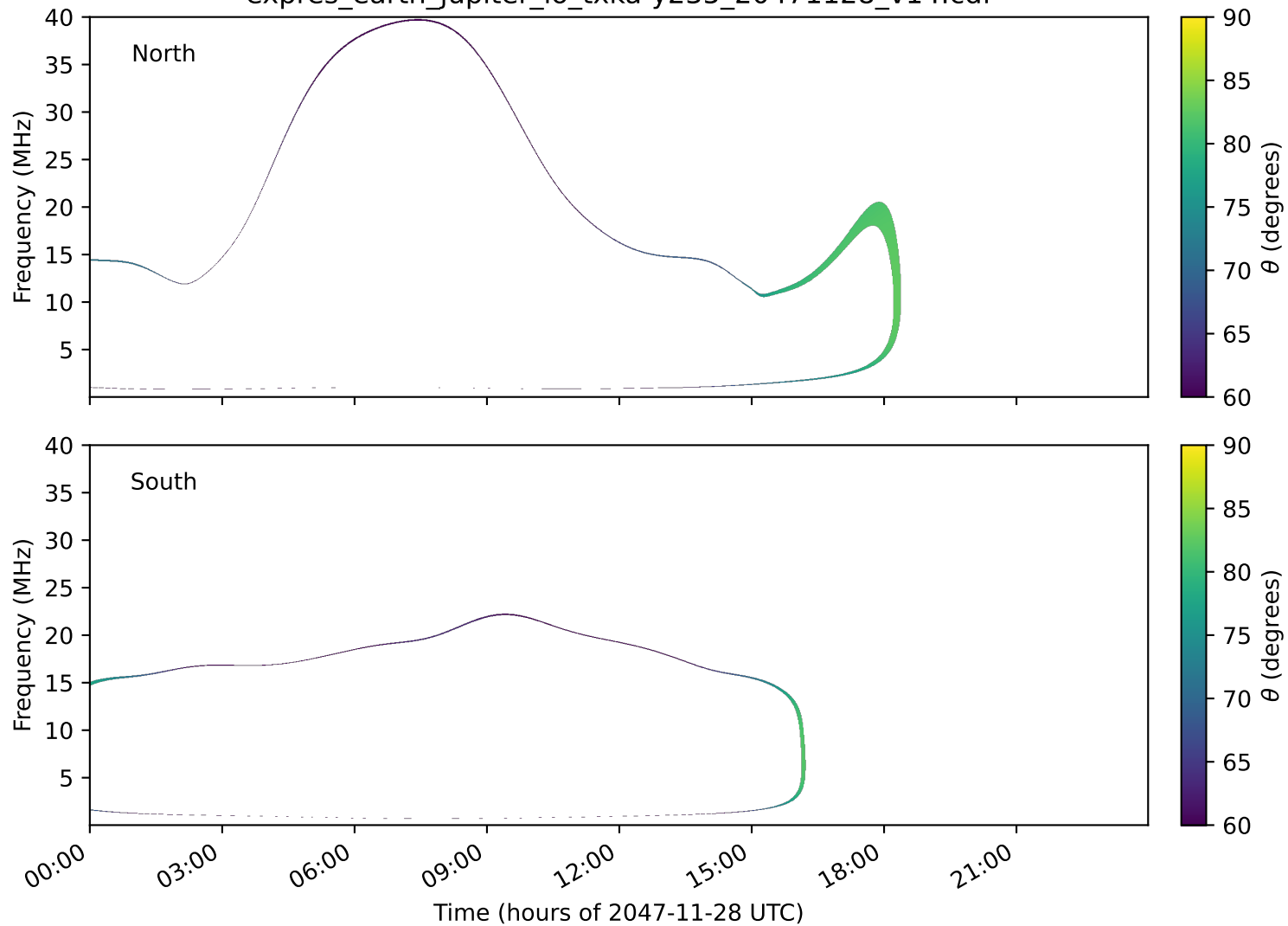
expres_earth_jupiter_io_txka-y235_20471128_v14.cdf
