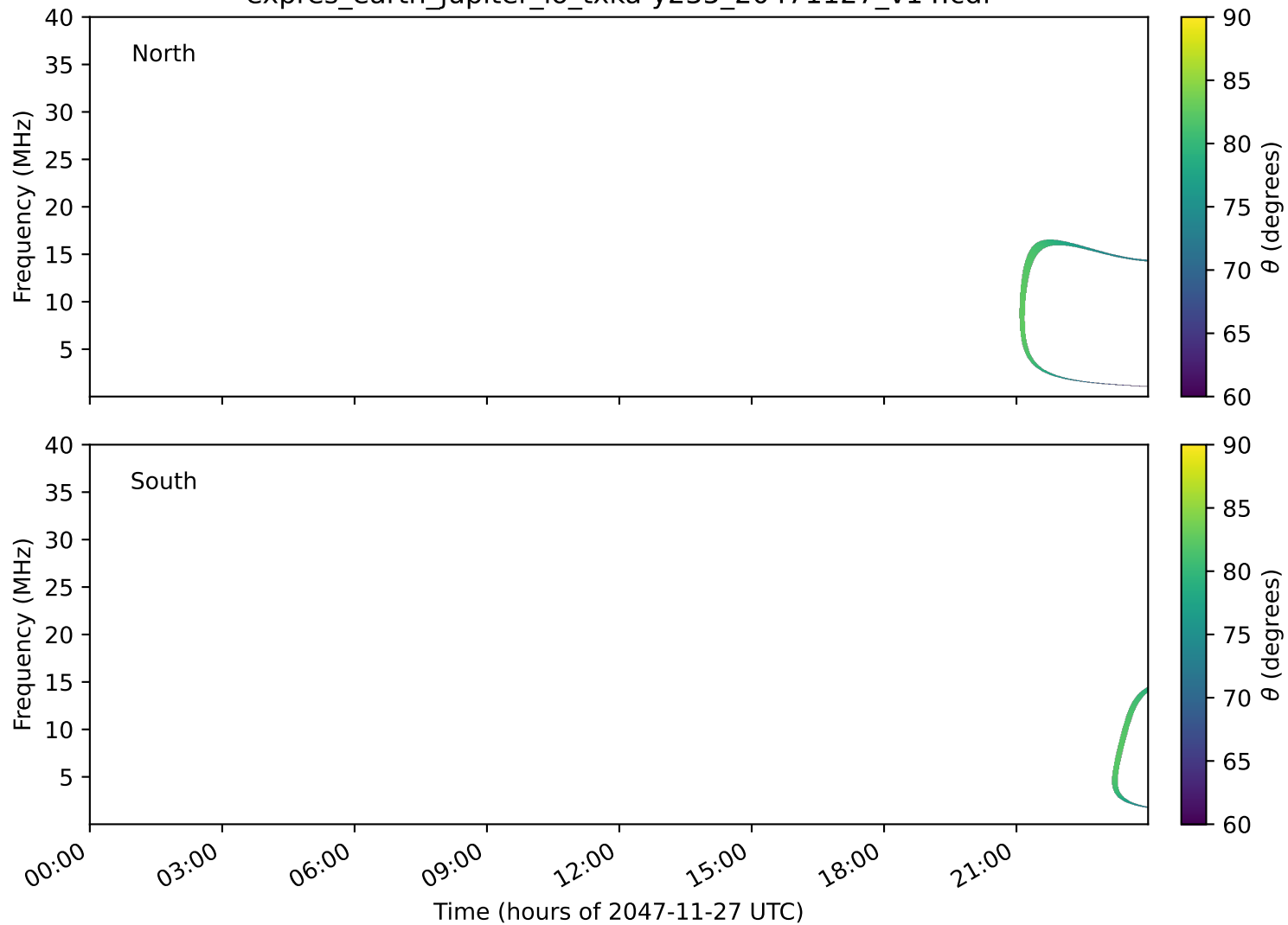
expres_earth_jupiter_io_txka-y235_20471127_v14.cdf
