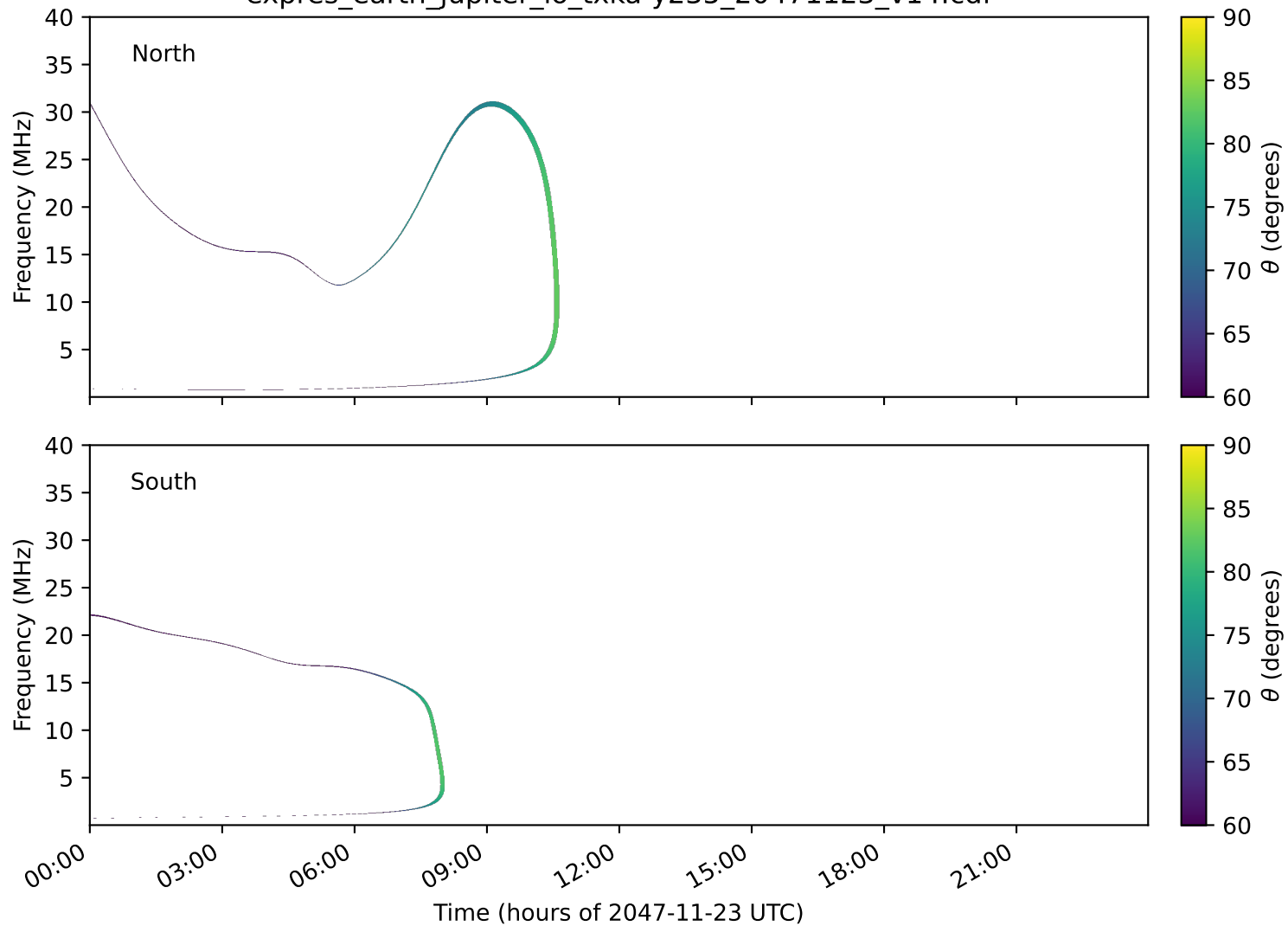
expres_earth_jupiter_io_txka-y235_20471123_v14.cdf
