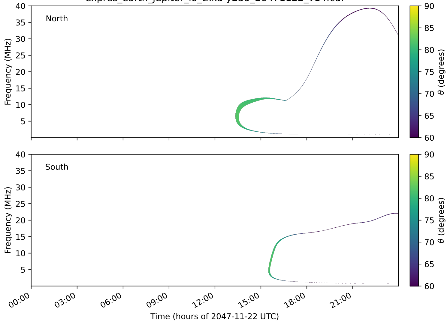
expres_earth_jupiter_io_txka-y235_20471122_v14.cdf
