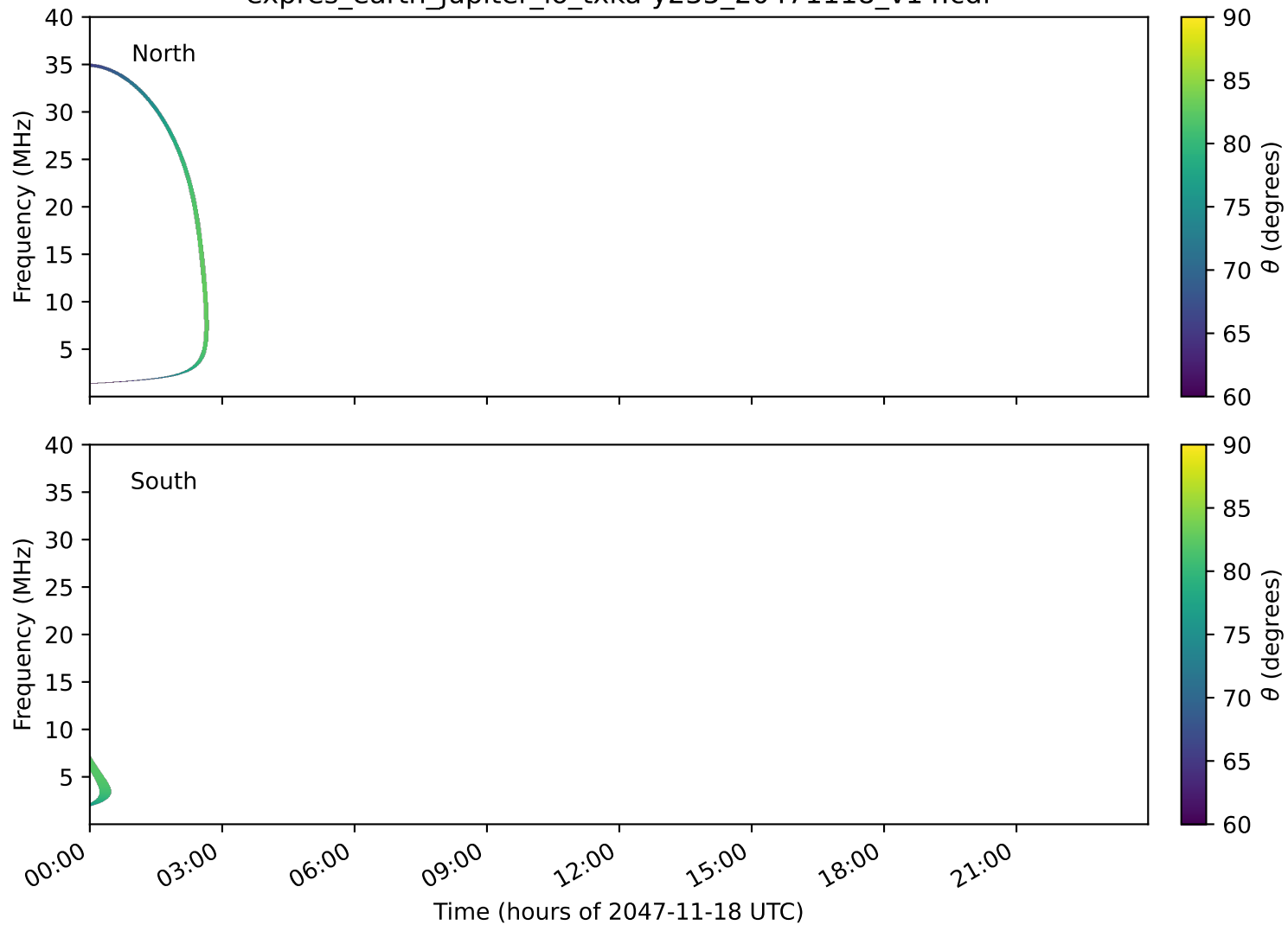
expres_earth_jupiter_io_txka-y235_20471118_v14.cdf
