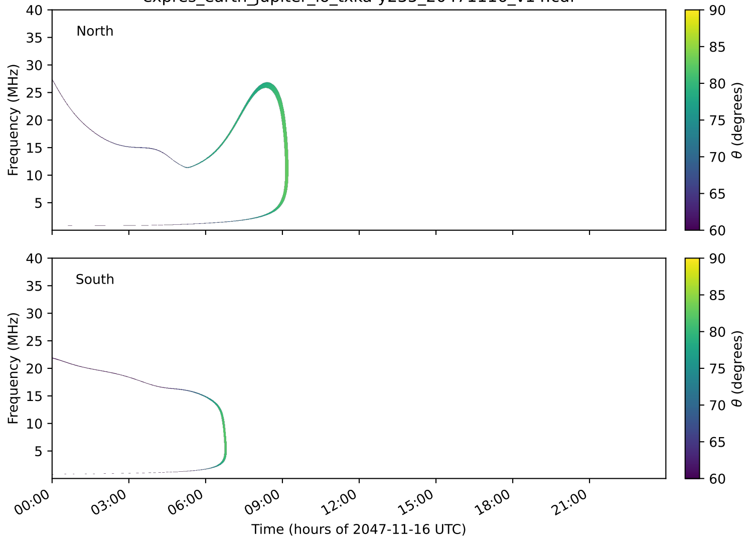
expres_earth_jupiter_io_txka-y235_20471116_v14.cdf
