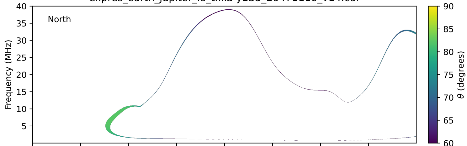
expres_earth_jupiter_io_txka-y235_20471110_v14.cdf
