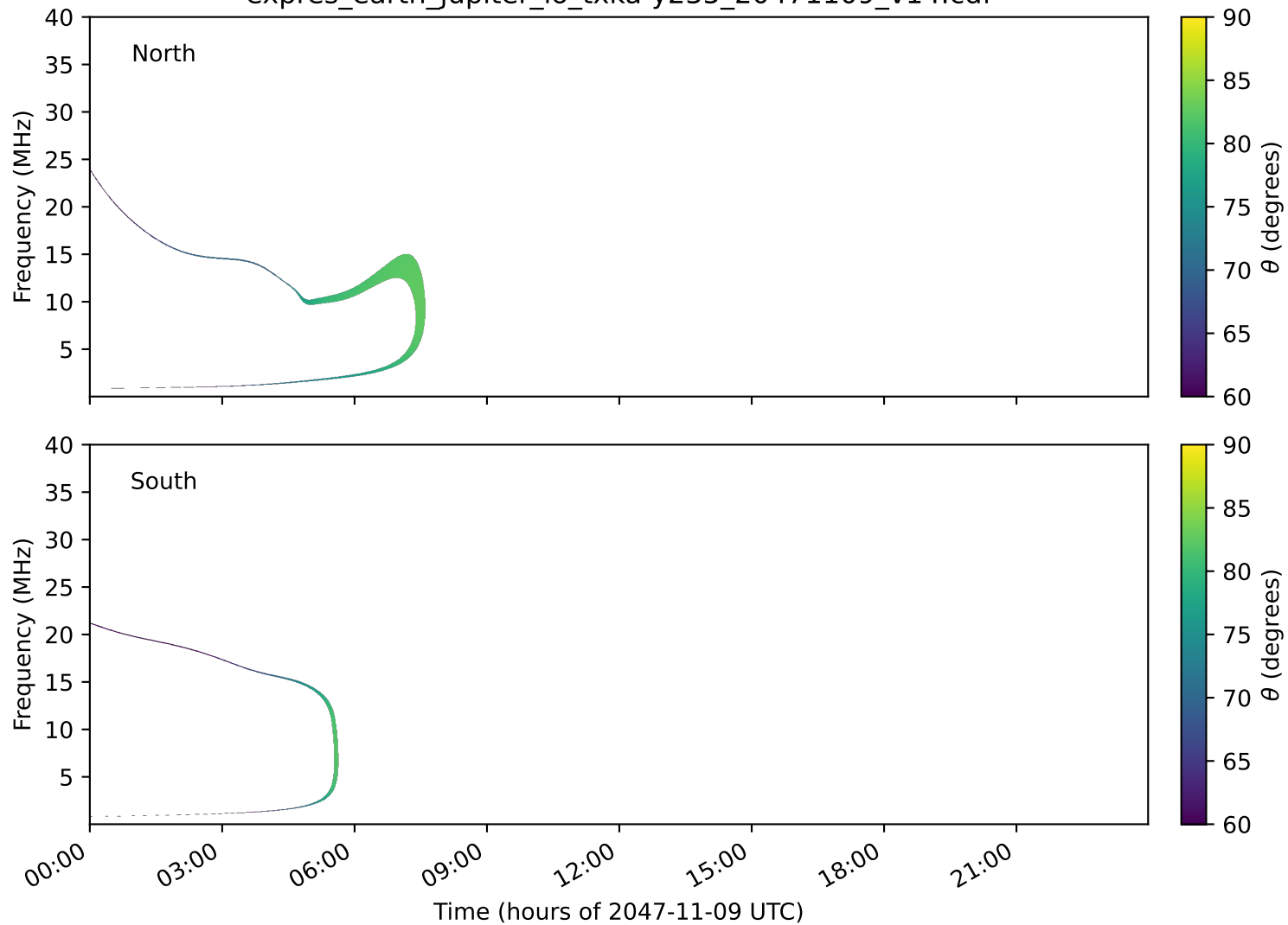
expres_earth_jupiter_io_txka-y235_20471109_v14.cdf
