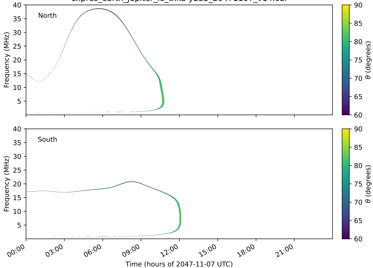
expres_earth_jupiter_io_txka-y235_20471107_v14.cdf
