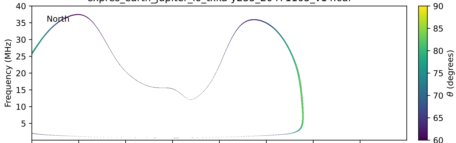
expres_earth_jupiter_io_txka-y235_20471105_v14.cdf
