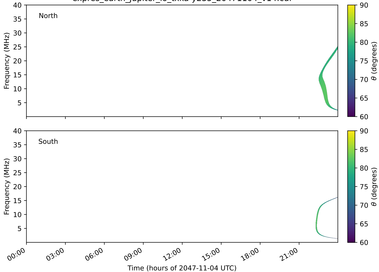
expres_earth_jupiter_io_txka-y235_20471104_v14.cdf
