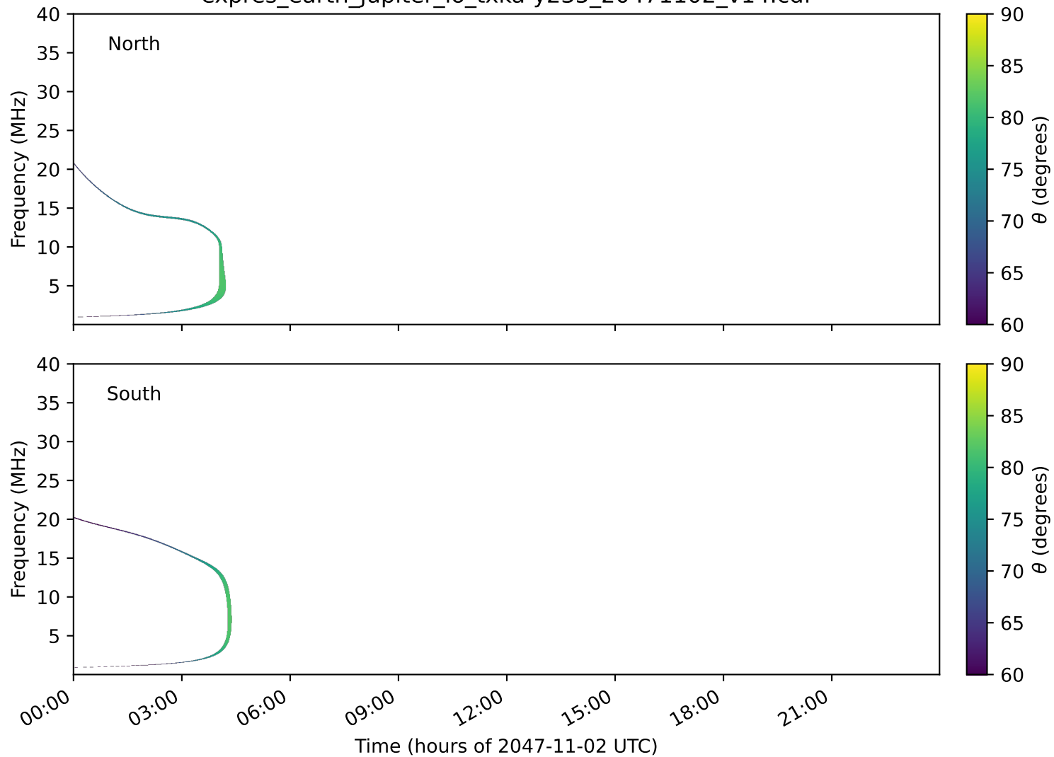
expres_earth_jupiter_io_txka-y235_20471102_v14.cdf
