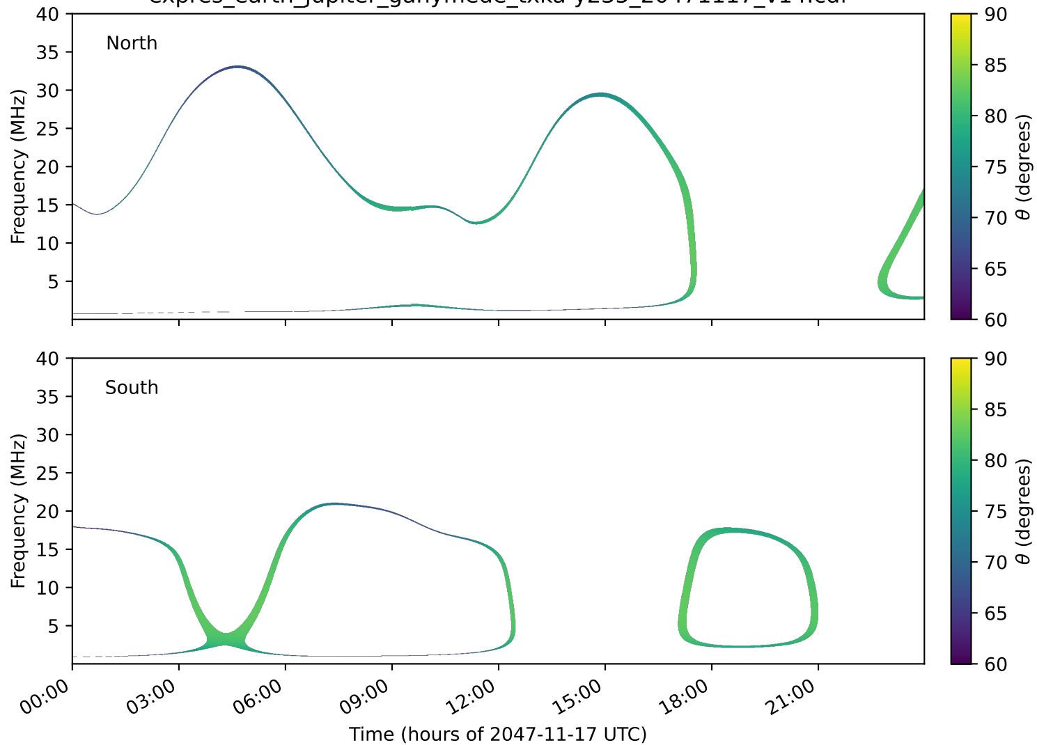
expres_earth_jupiter_ganymede_txka-y235_20471117_v14.cdf
