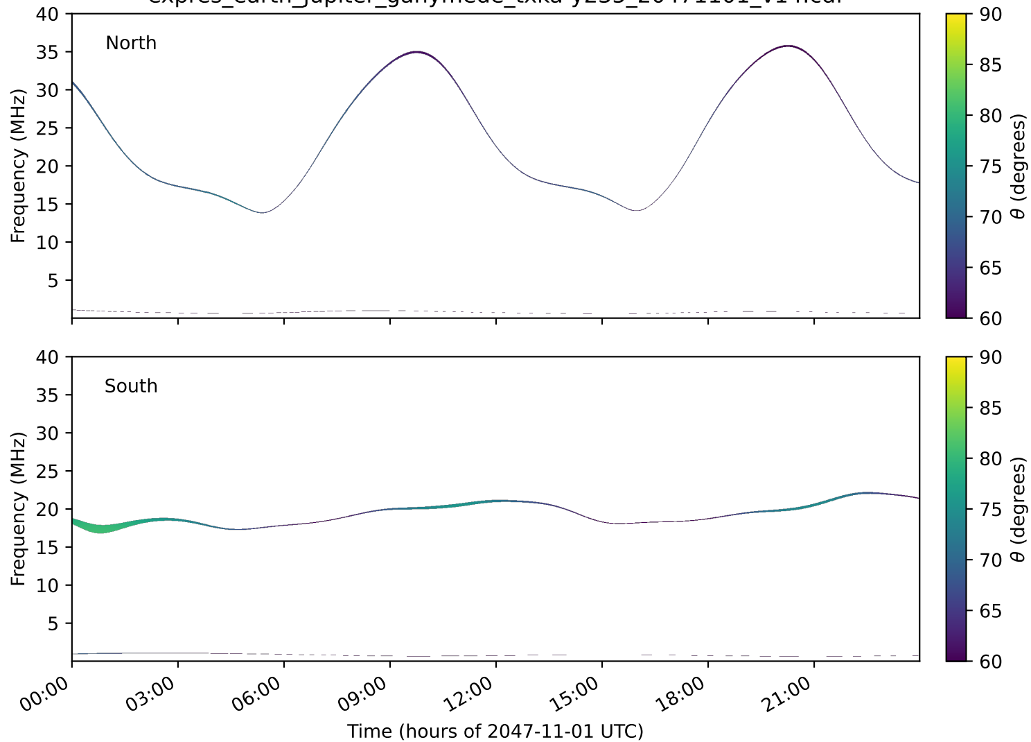
expres_earth_jupiter_ganymede_txka-y235_20471101_v14.cdf
