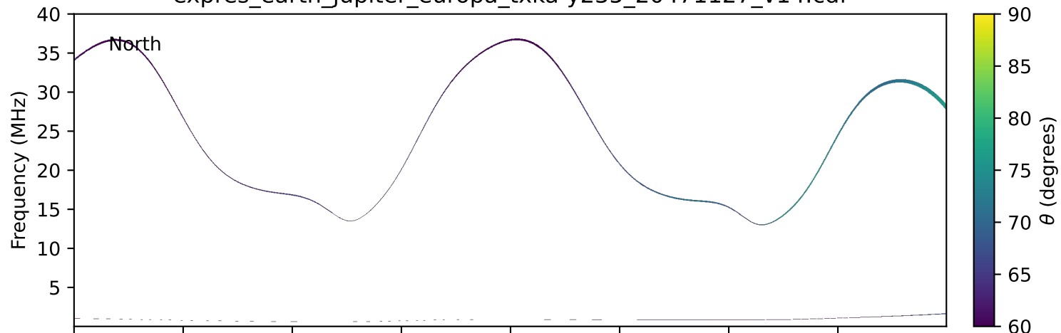
expres_earth_jupiter_europa_txka-y235_20471127_v14.cdf
