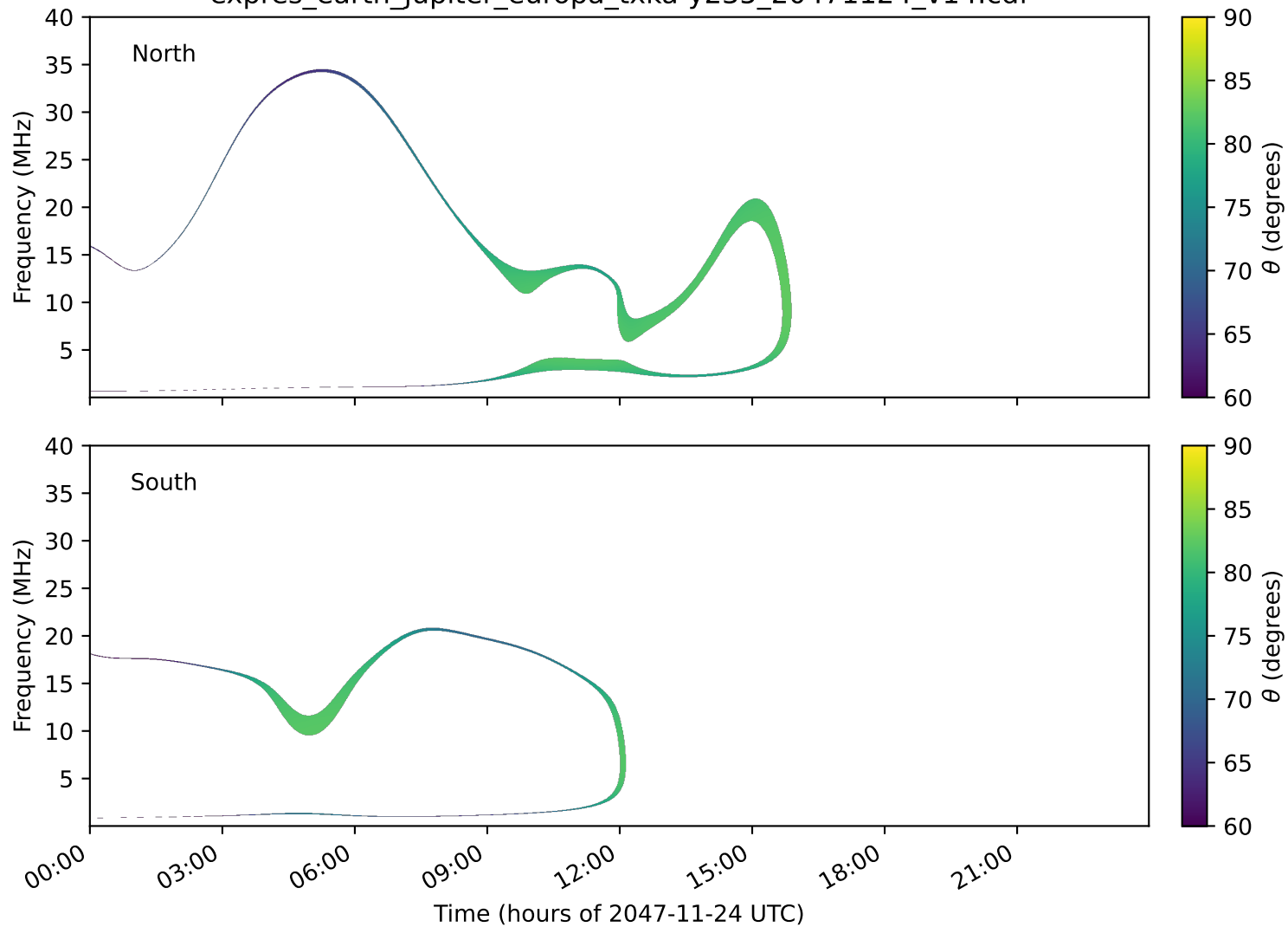
expres_earth_jupiter_europa_txka-y235_20471124_v14.cdf
