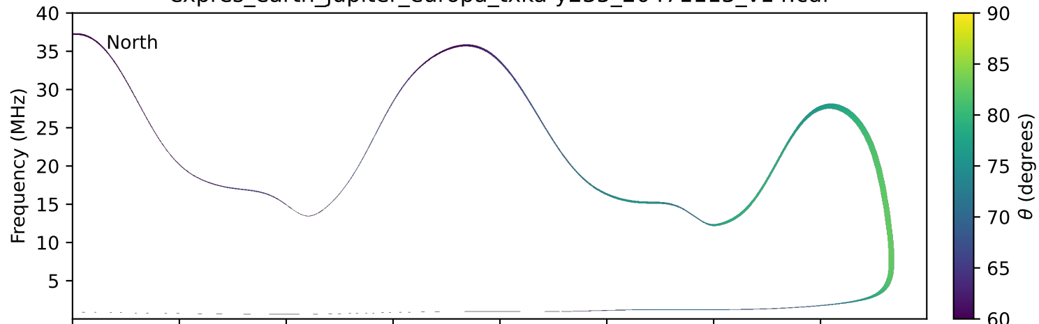
expres_earth_jupiter_europa_txka-y235_20471113_v14.cdf
