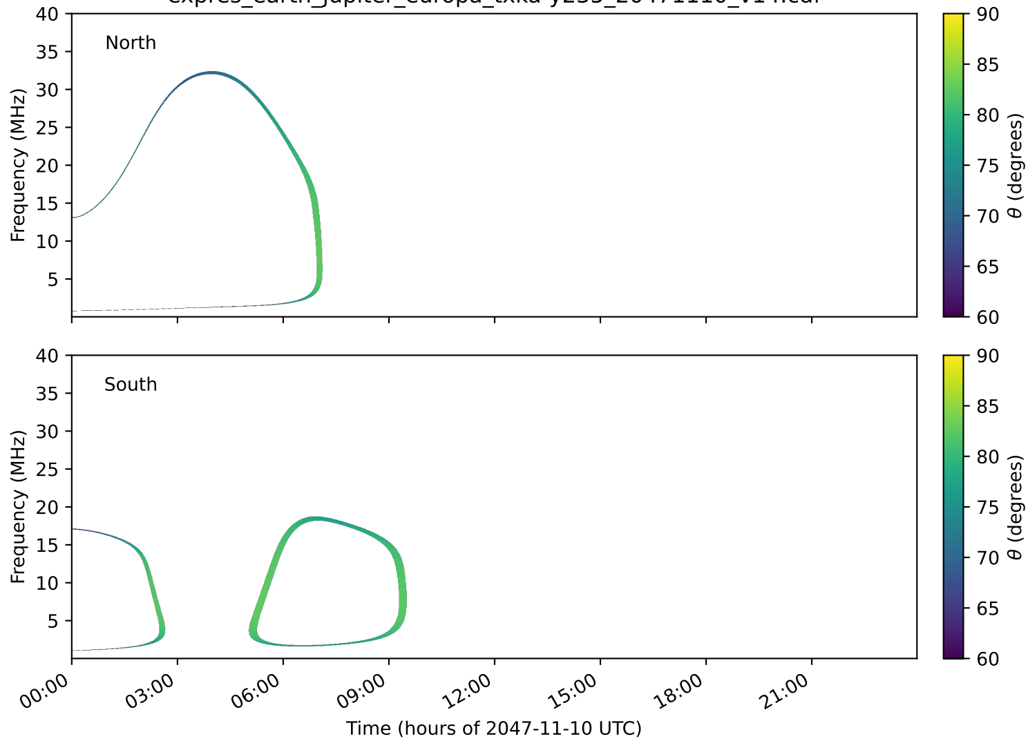
expres_earth_jupiter_europa_txka-y235_20471110_v14.cdf
