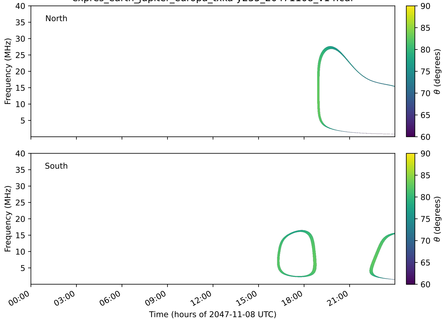
expres_earth_jupiter_europa_txka-y235_20471108_v14.cdf
