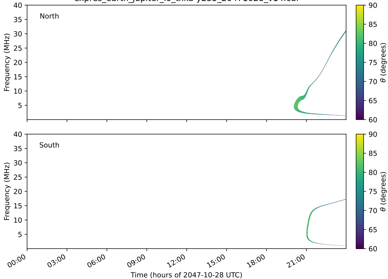
expres_earth_jupiter_io_txka-y235_20471028_v14.cdf
