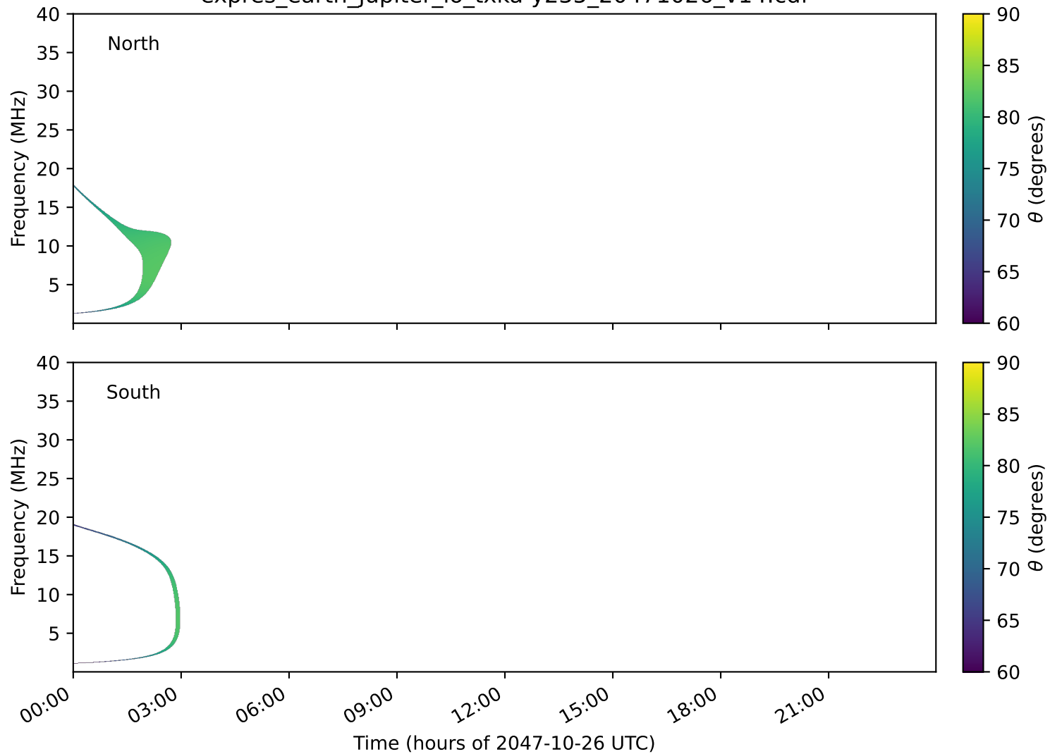
expres_earth_jupiter_io_txka-y235_20471026_v14.cdf
