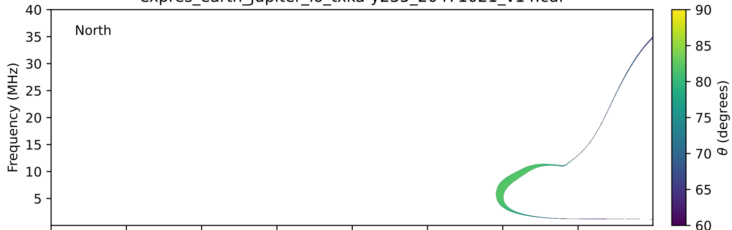
expres_earth_jupiter_io_txka-y235_20471021_v14.cdf
