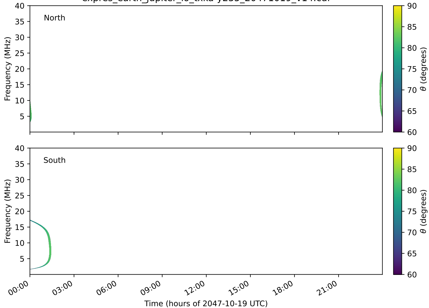
expres_earth_jupiter_io_txka-y235_20471019_v14.cdf
