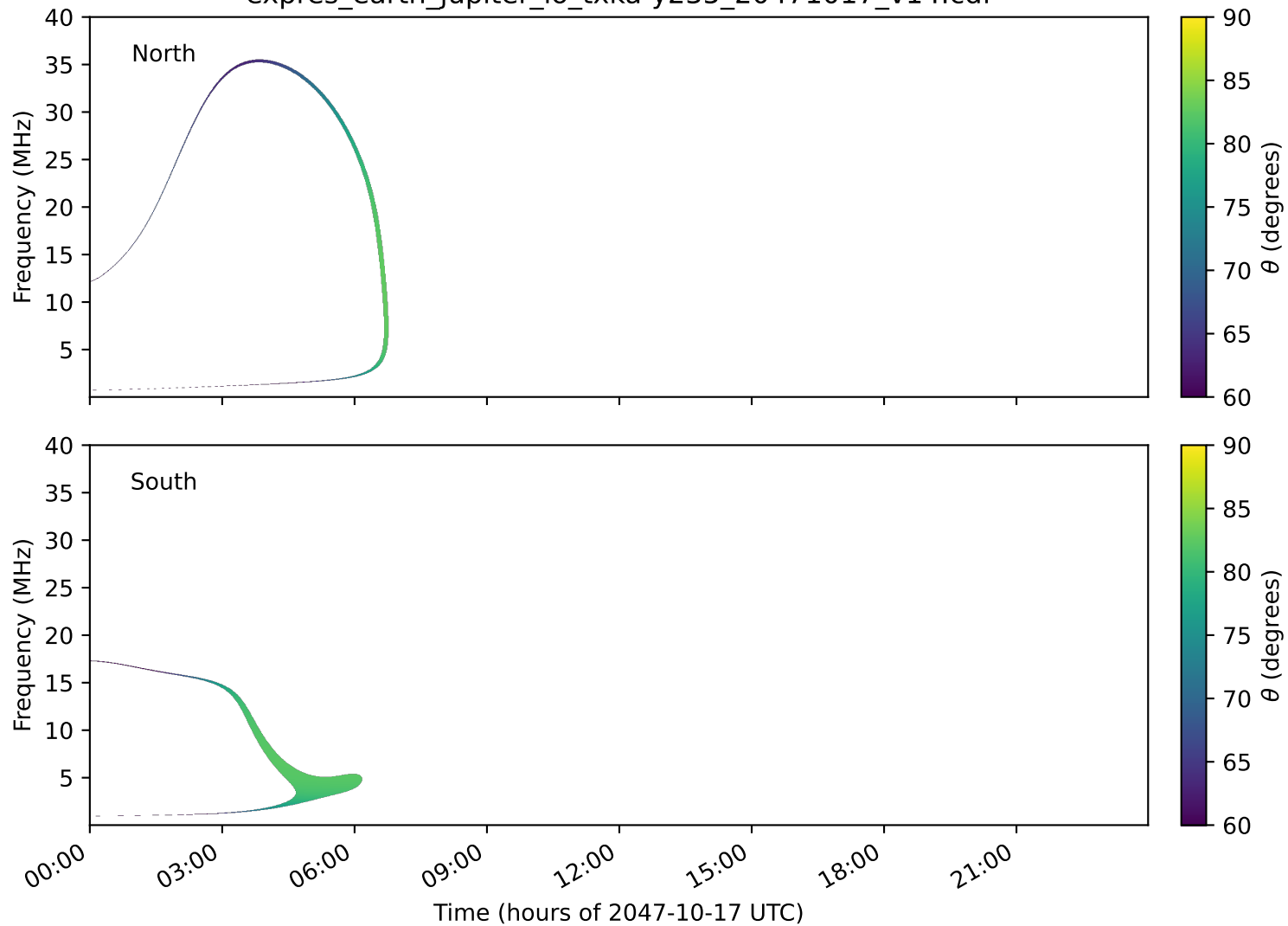
expres_earth_jupiter_io_txka-y235_20471017_v14.cdf
