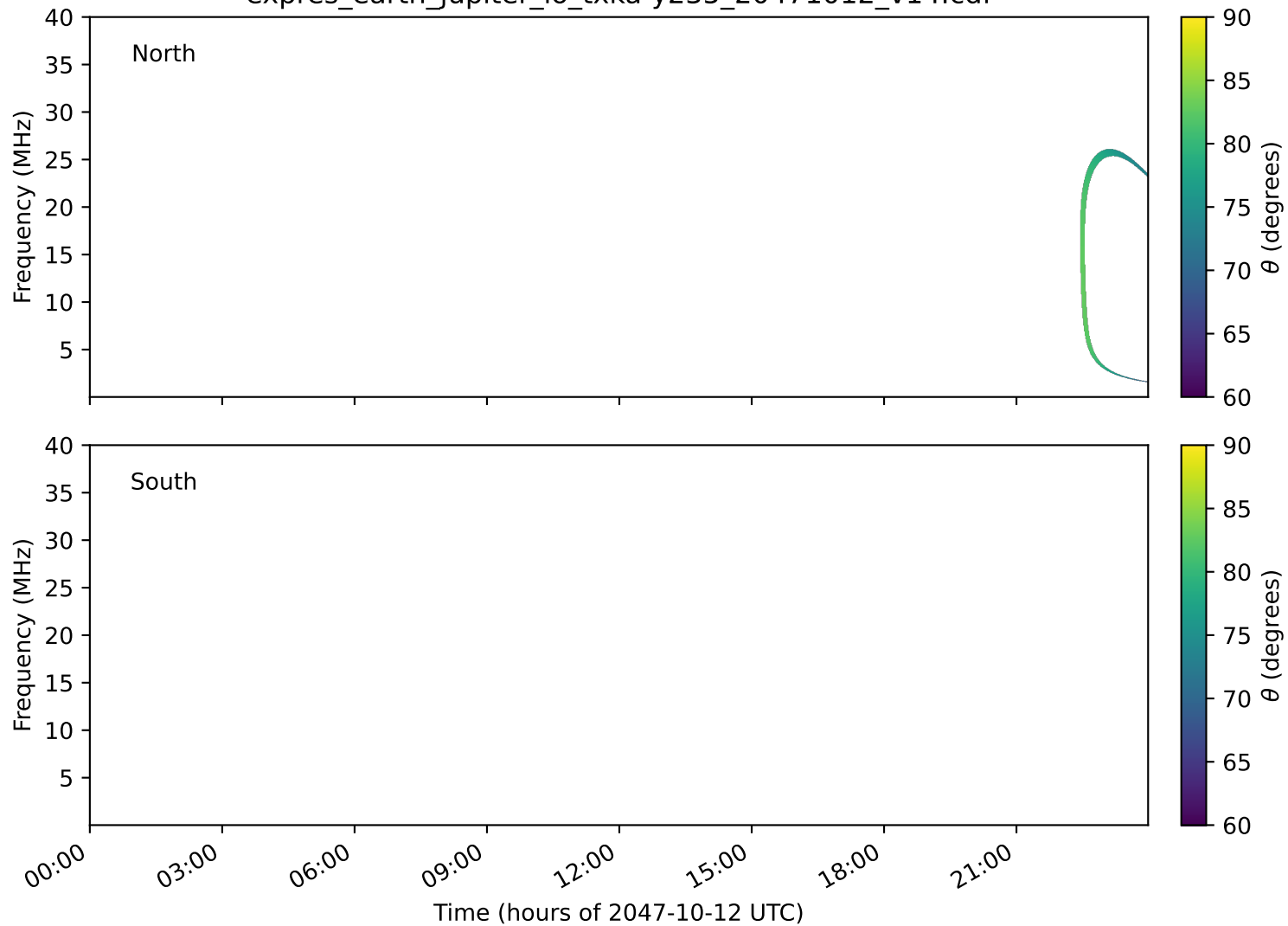
expres_earth_jupiter_io_txka-y235_20471012_v14.cdf
