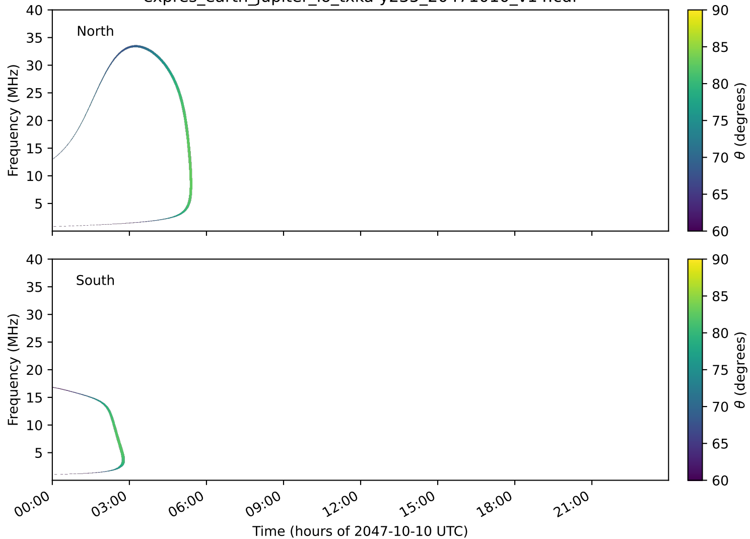
expres_earth_jupiter_io_txka-y235_20471010_v14.cdf
