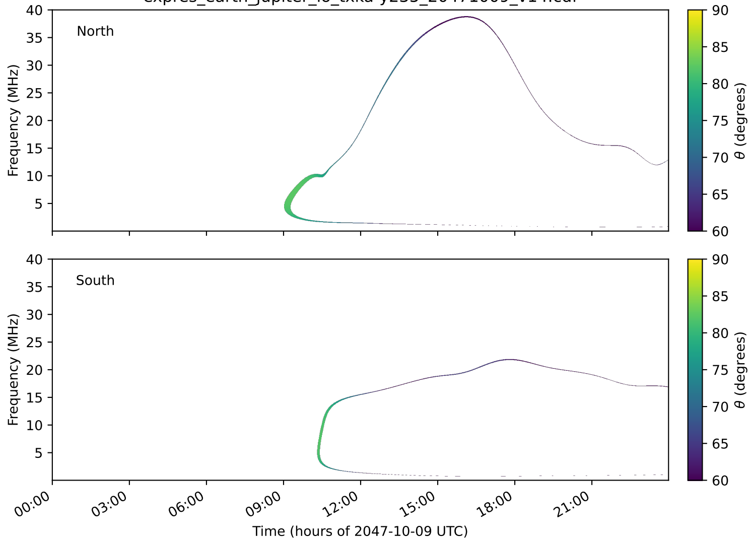
expres_earth_jupiter_io_txka-y235_20471009_v14.cdf
