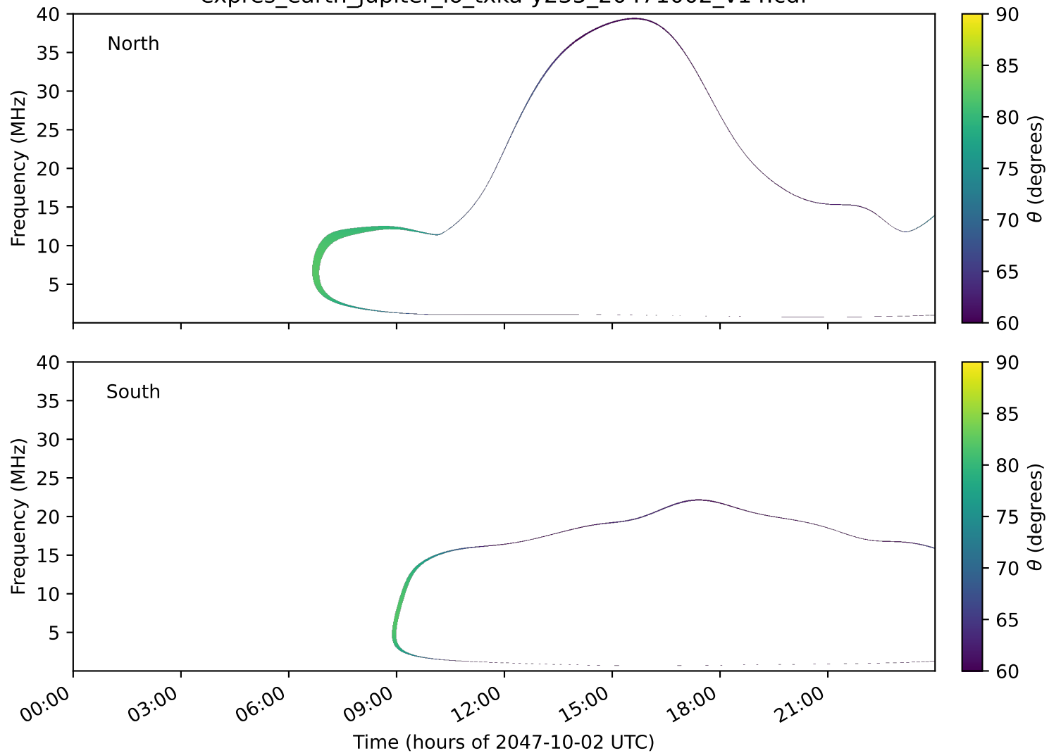
expres_earth_jupiter_io_txka-y235_20471002_v14.cdf
