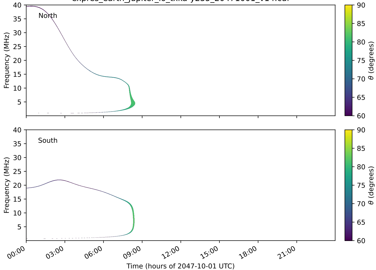
expres_earth_jupiter_io_txka-y235_20471001_v14.cdf
