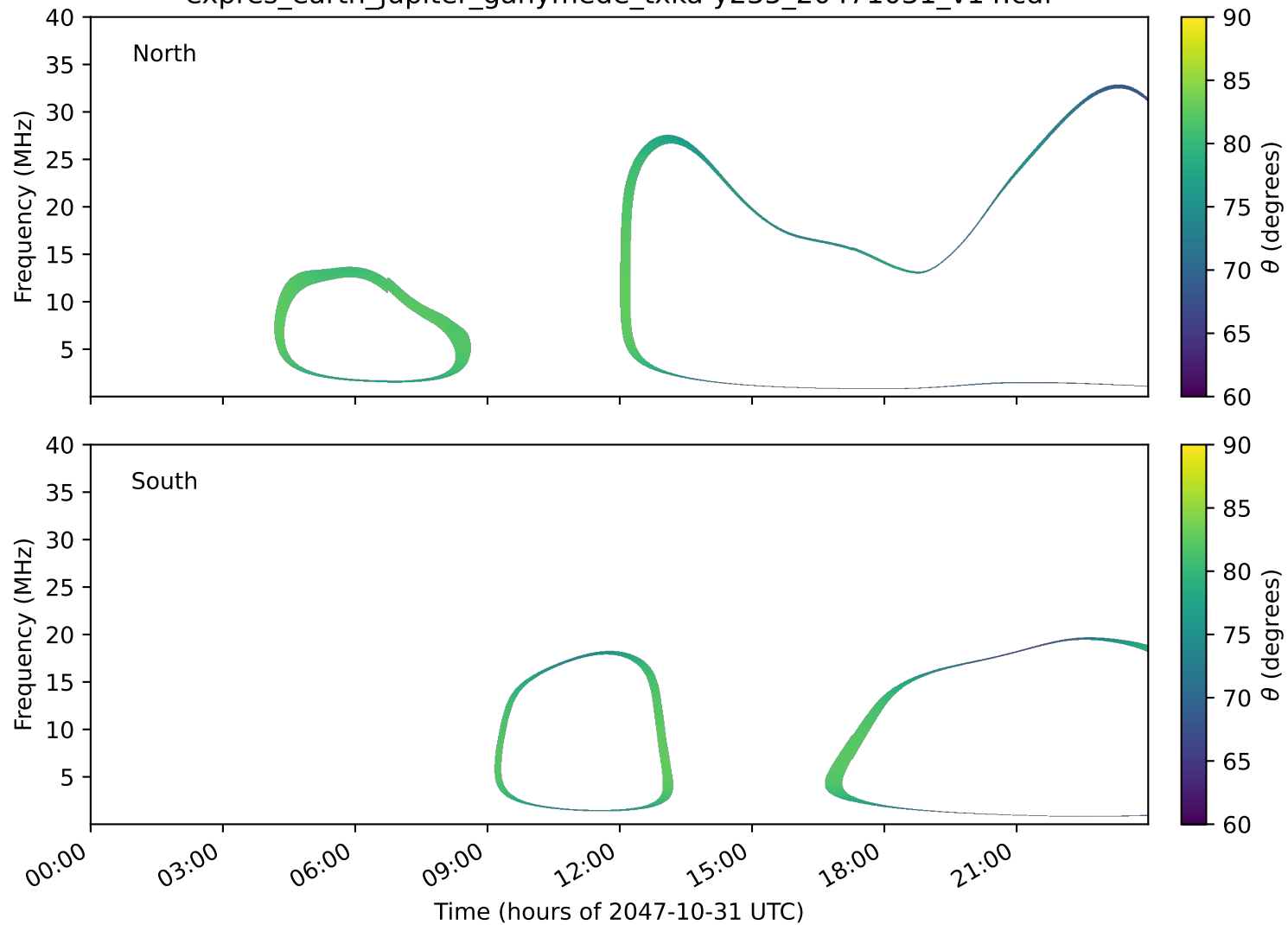
expres_earth_jupiter_ganymede_txka-y235_20471031_v14.cdf
