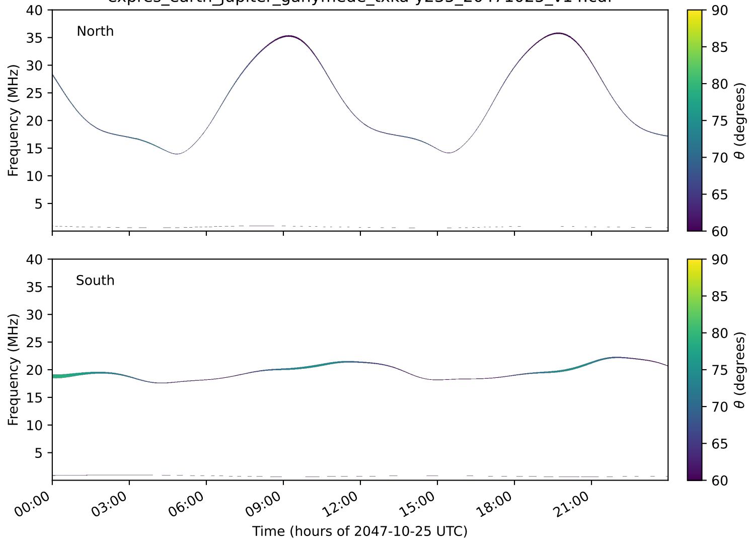
expres_earth_jupiter_ganymede_txka-y235_20471025_v14.cdf
