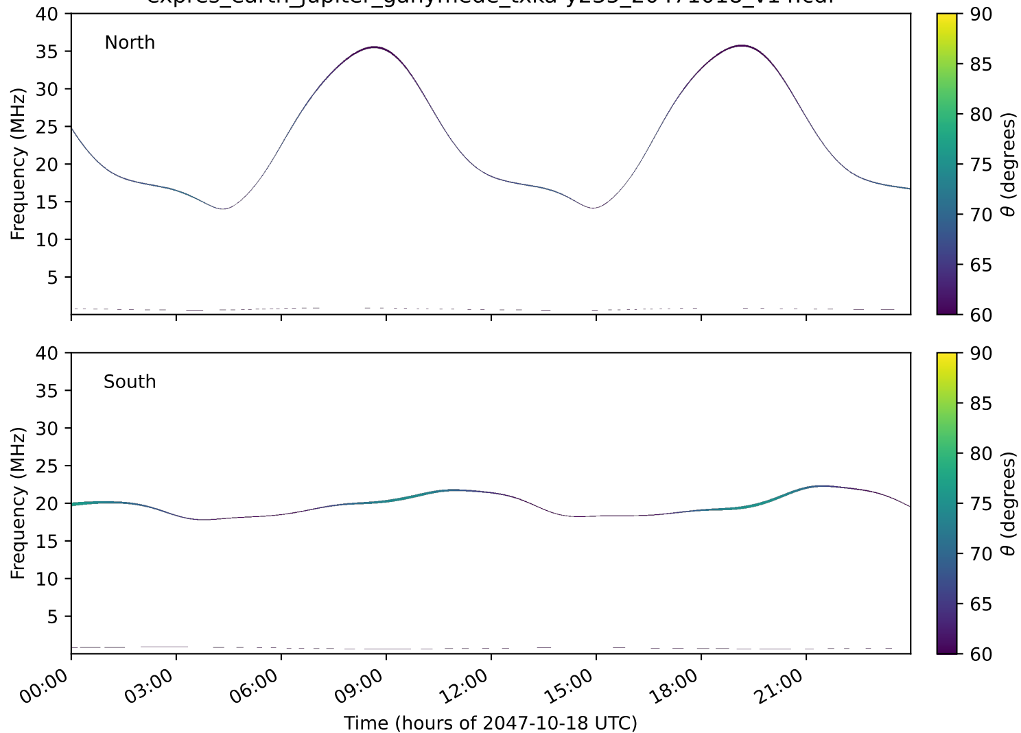
expres_earth_jupiter_ganymede_txka-y235_20471018_v14.cdf
