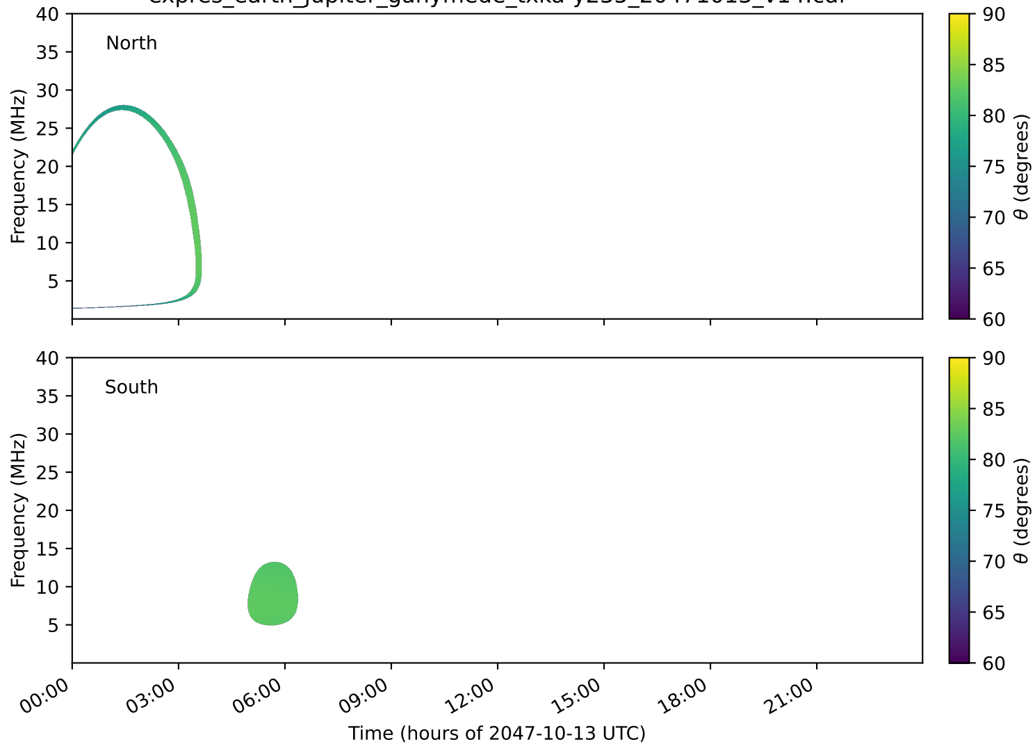
expres_earth_jupiter_ganymede_txka-y235_20471013_v14.cdf
