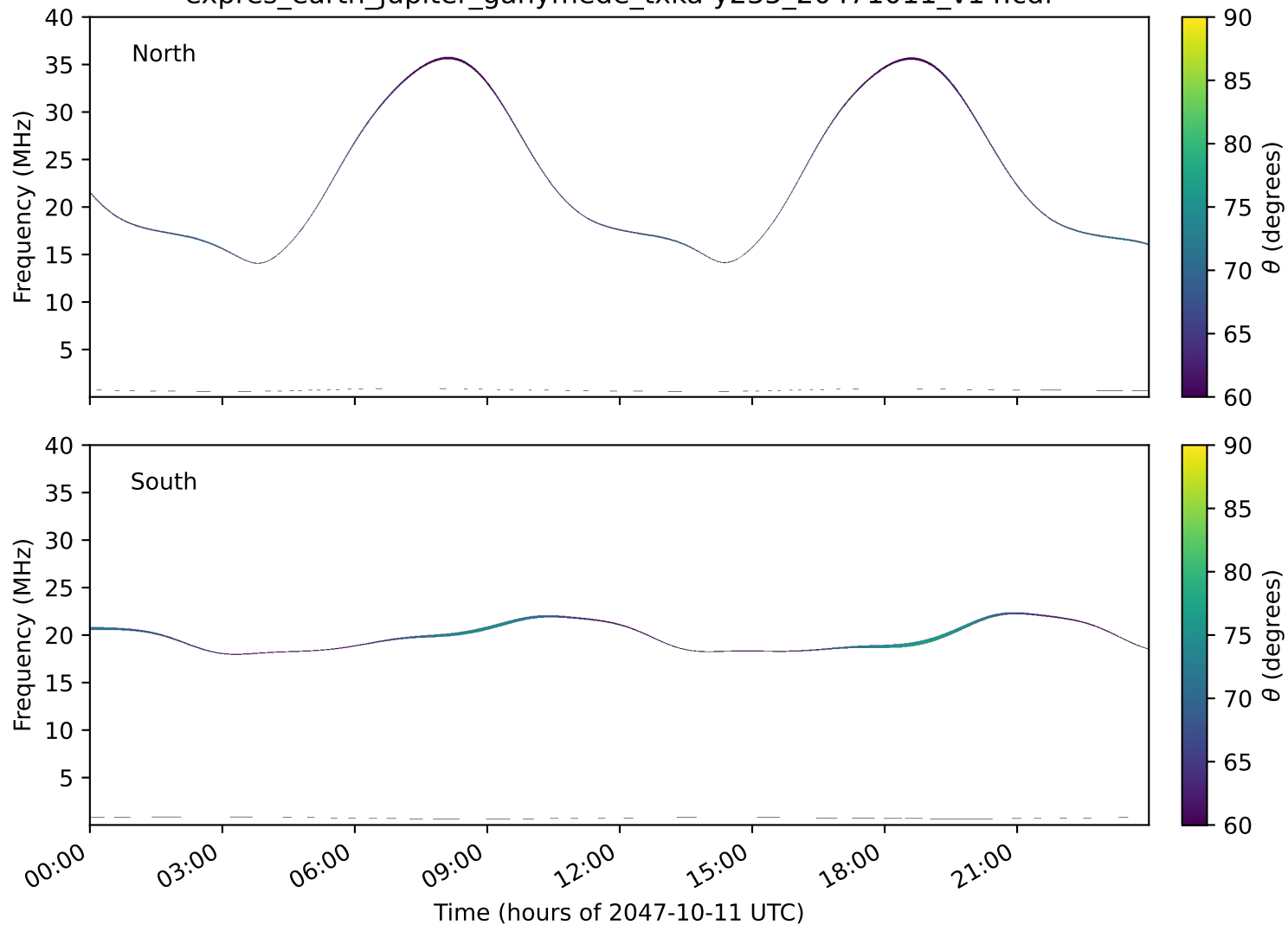
expres_earth_jupiter_ganymede_txka-y235_20471011_v14.cdf
