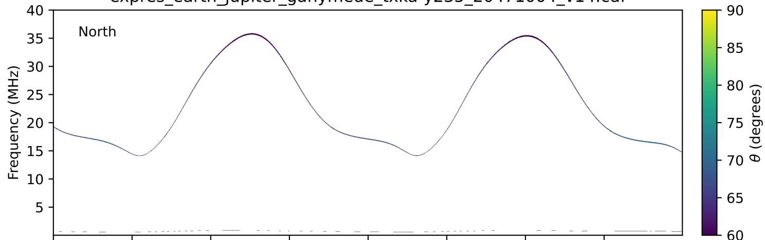
expres_earth_jupiter_ganymede_txka-y235_20471004_v14.cdf
