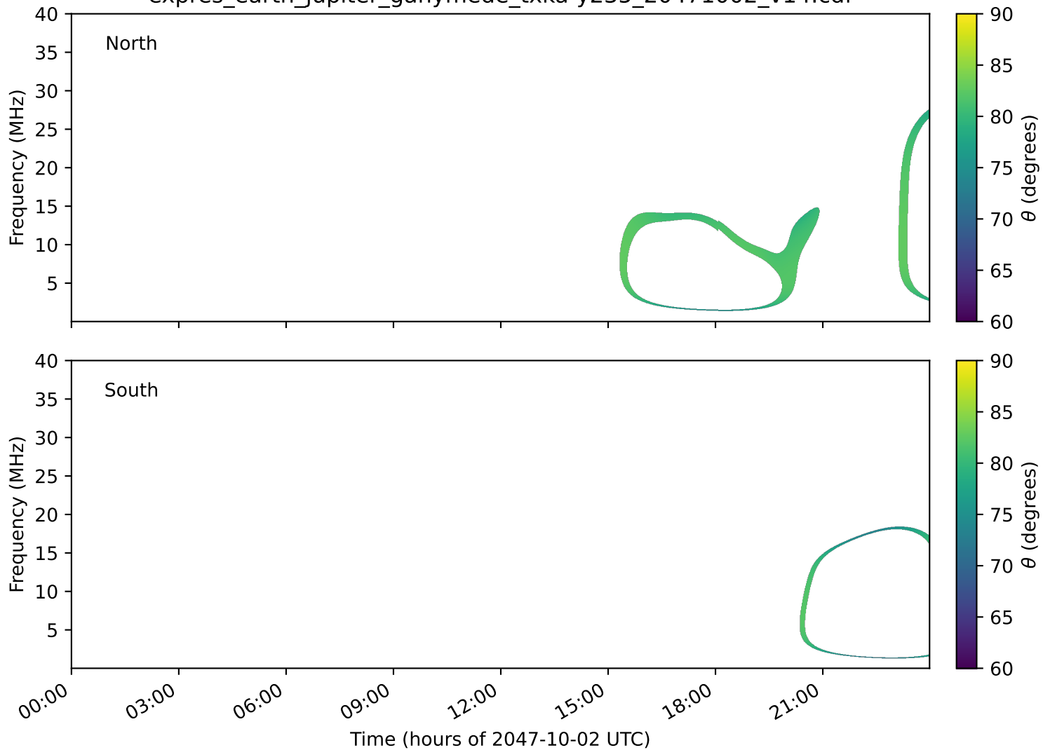
expres_earth_jupiter_ganymede_txka-y235_20471002_v14.cdf
