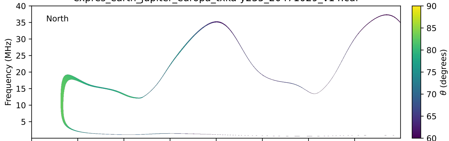
expres_earth_jupiter_europa_txka-y235_20471029_v14.cdf
