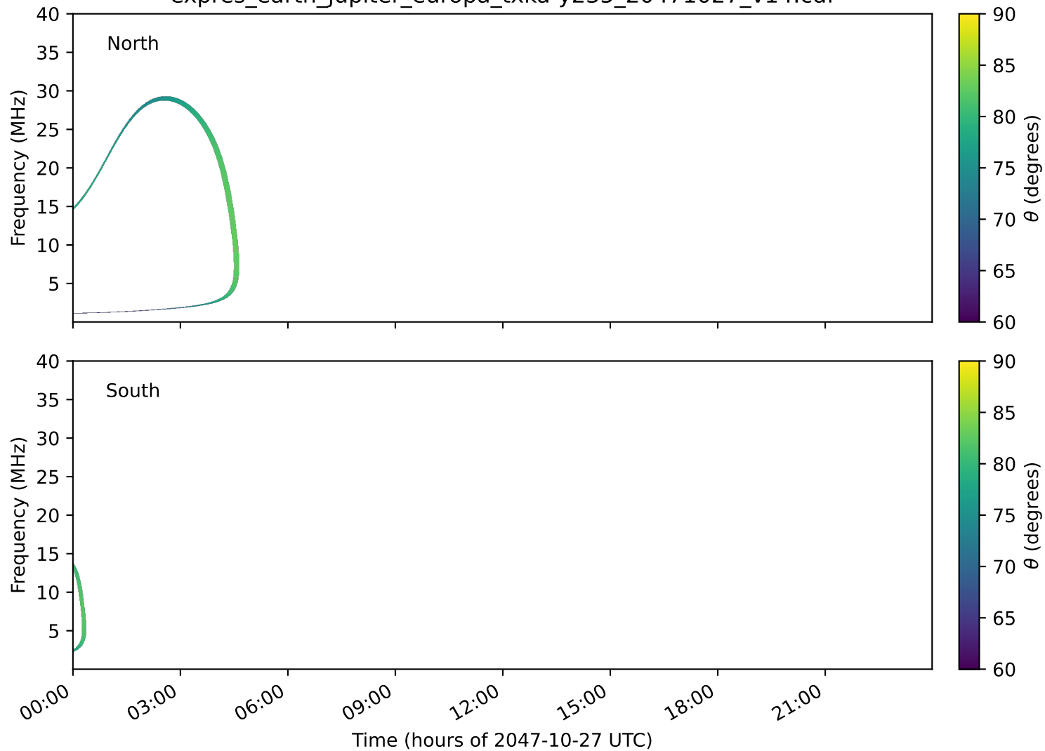
expres_earth_jupiter_europa_txka-y235_20471027_v14.cdf
