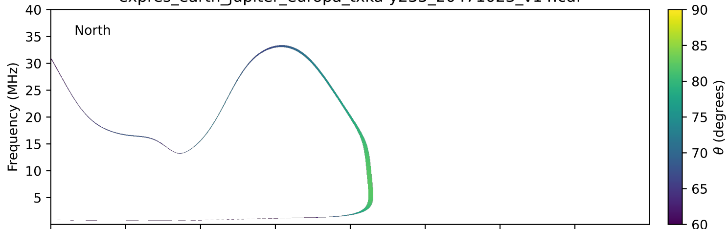
expres_earth_jupiter_europa_txka-y235_20471023_v14.cdf
