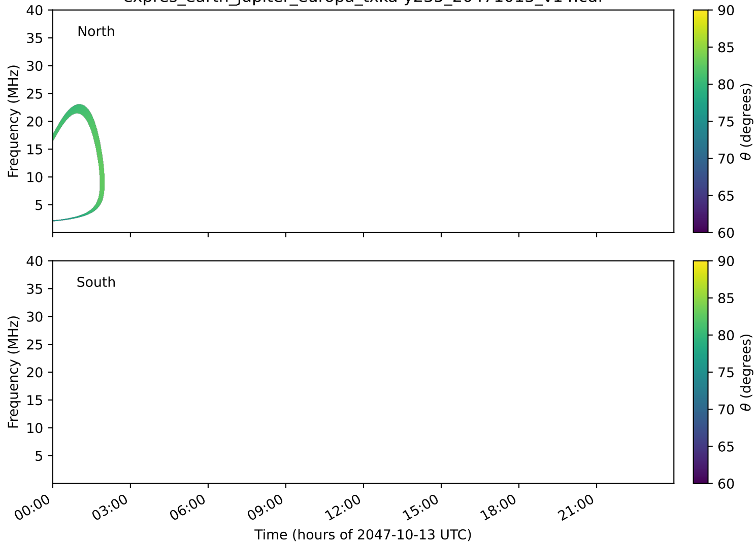
expres_earth_jupiter_europa_txka-y235_20471013_v14.cdf
