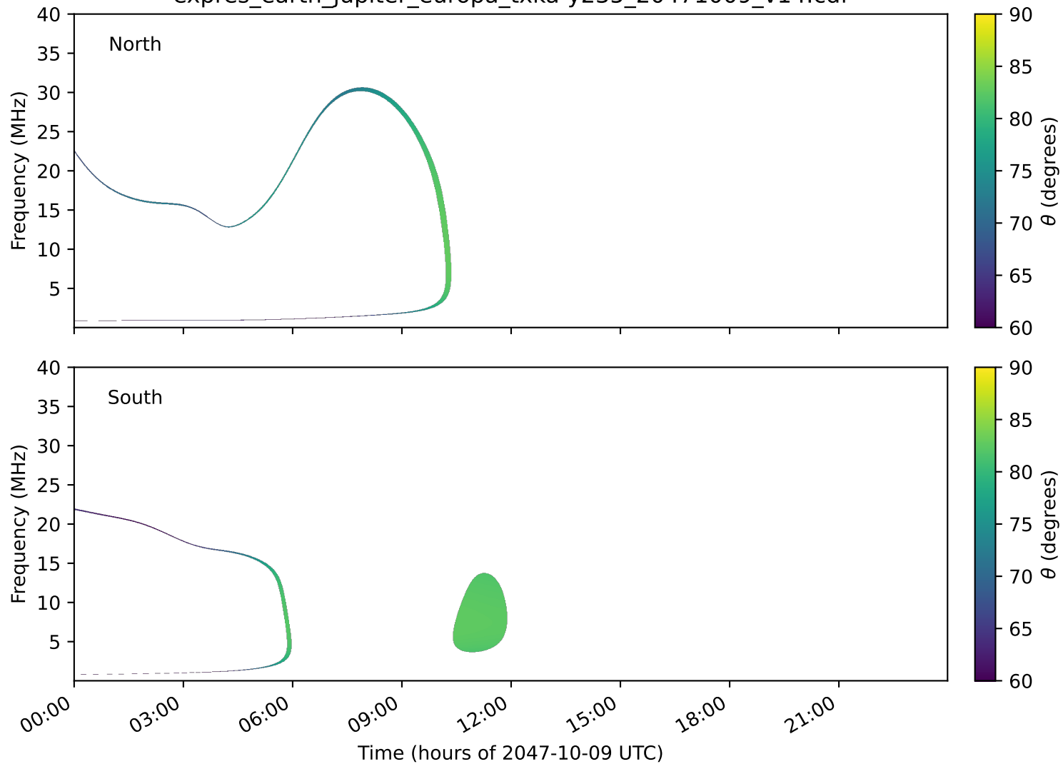
expres_earth_jupiter_europa_txka-y235_20471009_v14.cdf
