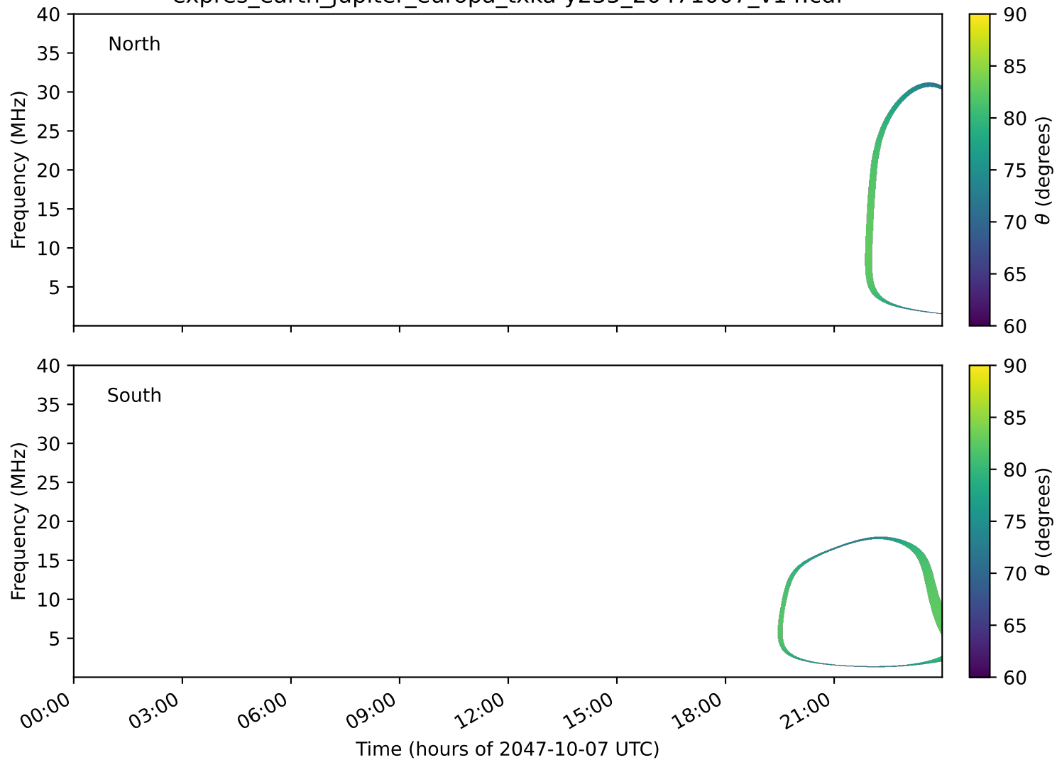
expres_earth_jupiter_europa_txka-y235_20471007_v14.cdf
