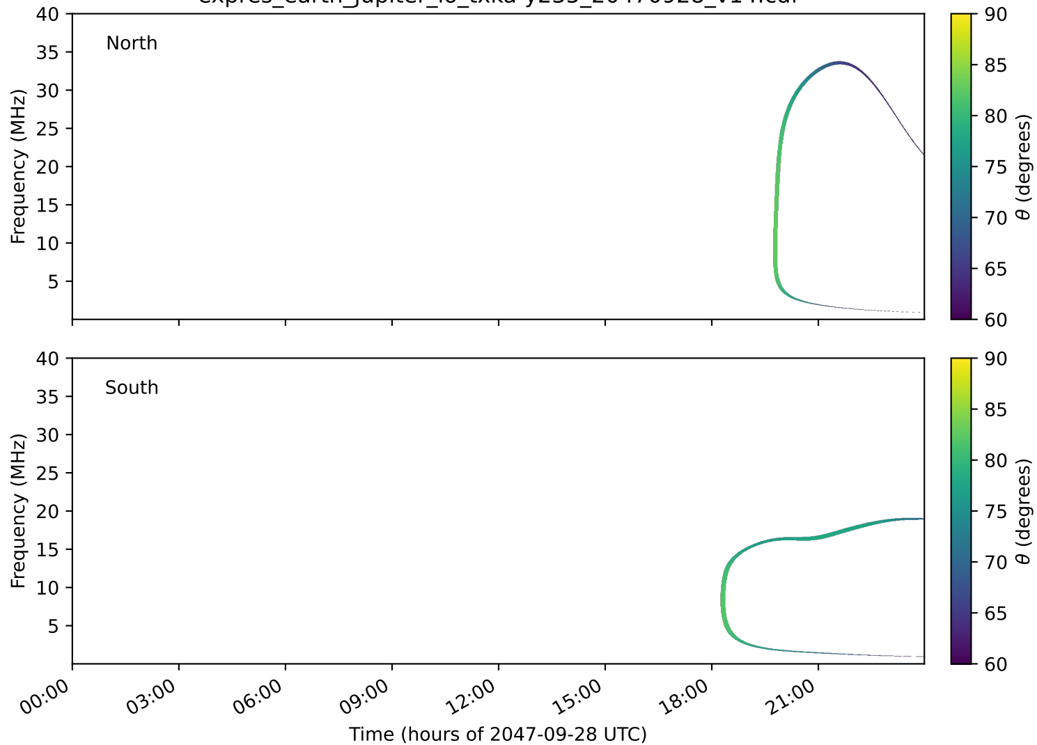
expres_earth_jupiter_io_txka-y235_20470928_v14.cdf
