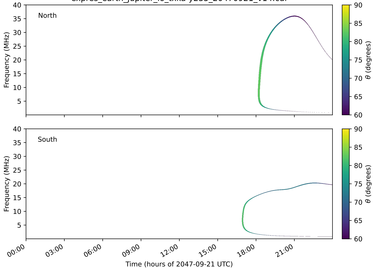
expres_earth_jupiter_io_txka-y235_20470921_v14.cdf
