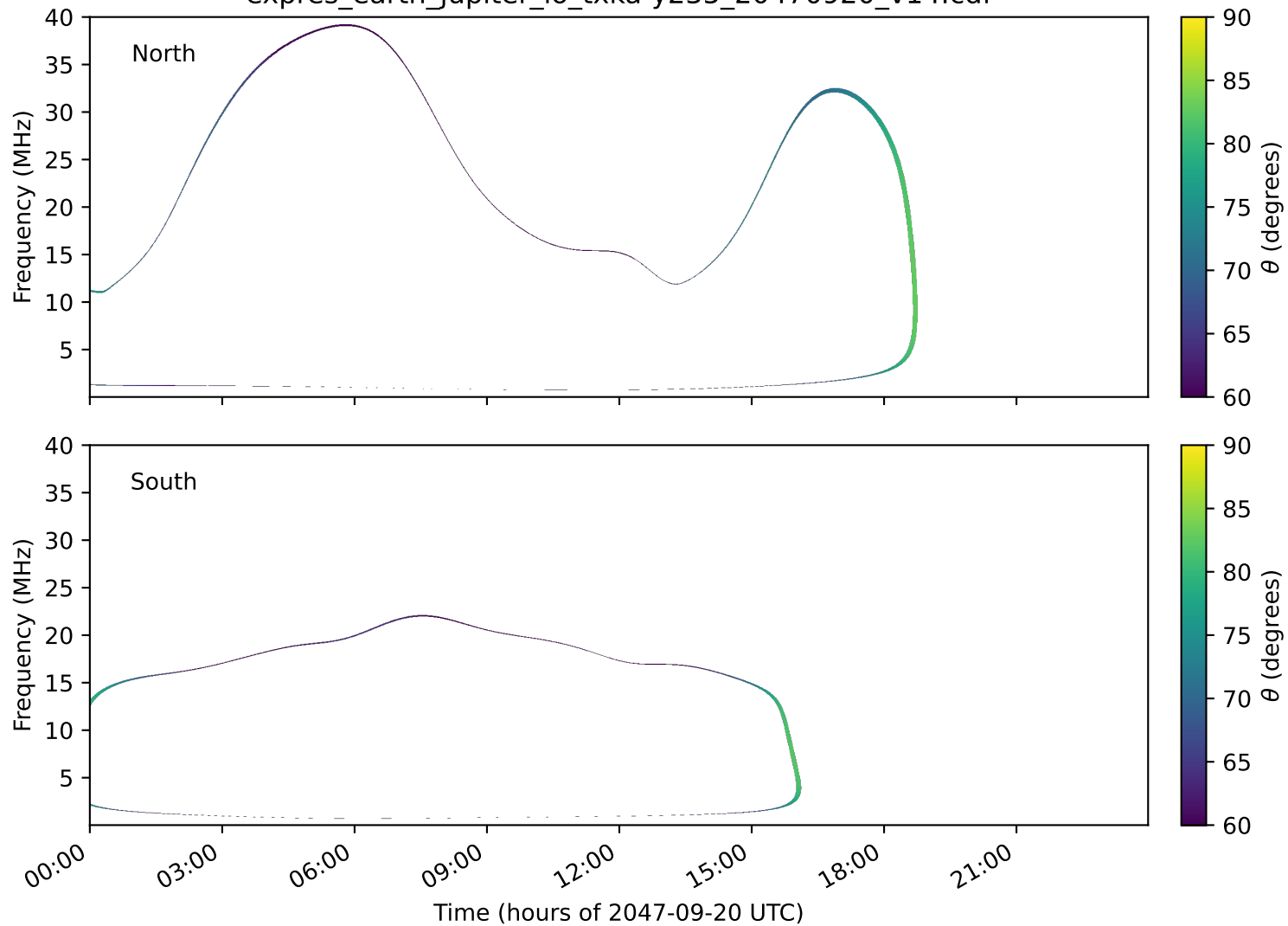
expres_earth_jupiter_io_txka-y235_20470920_v14.cdf
