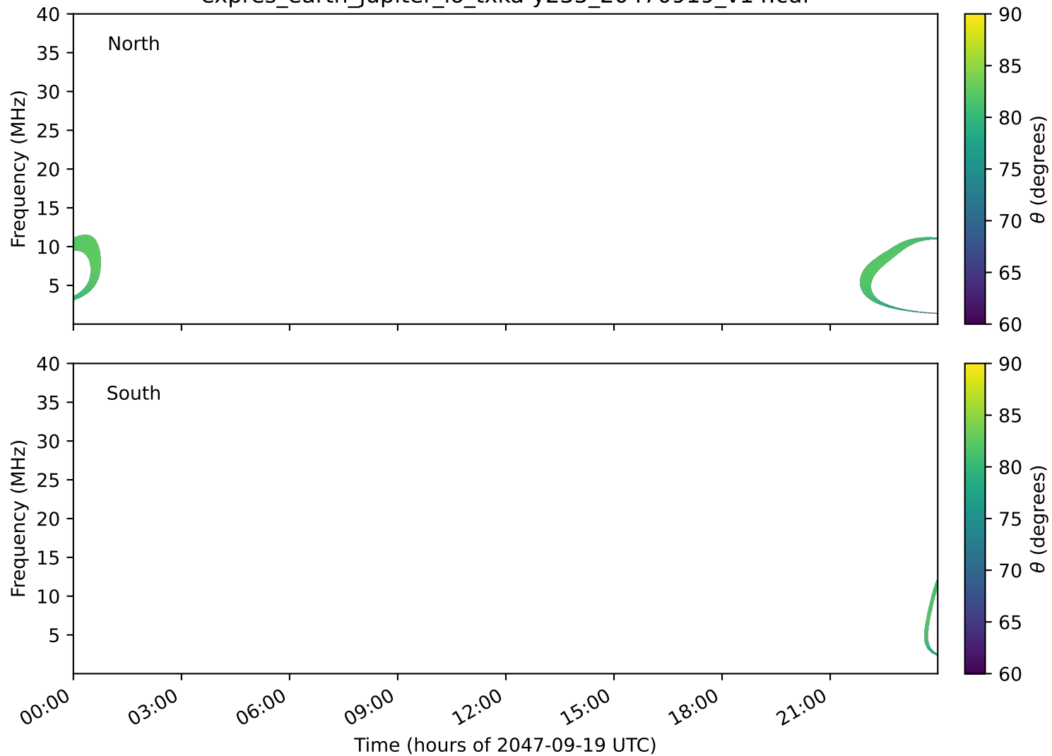
expres_earth_jupiter_io_txka-y235_20470919_v14.cdf
